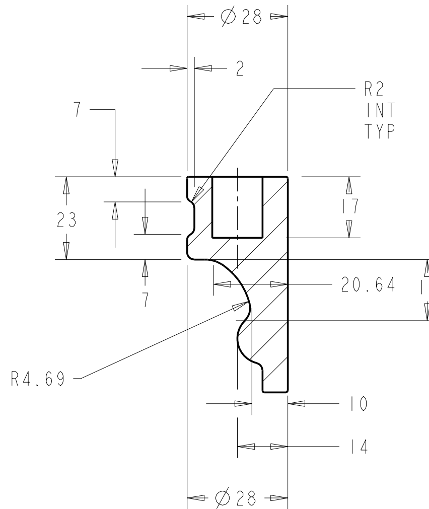
SECTION Z-Z
